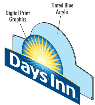
Assembly View of the Layers (hardware not shown)
